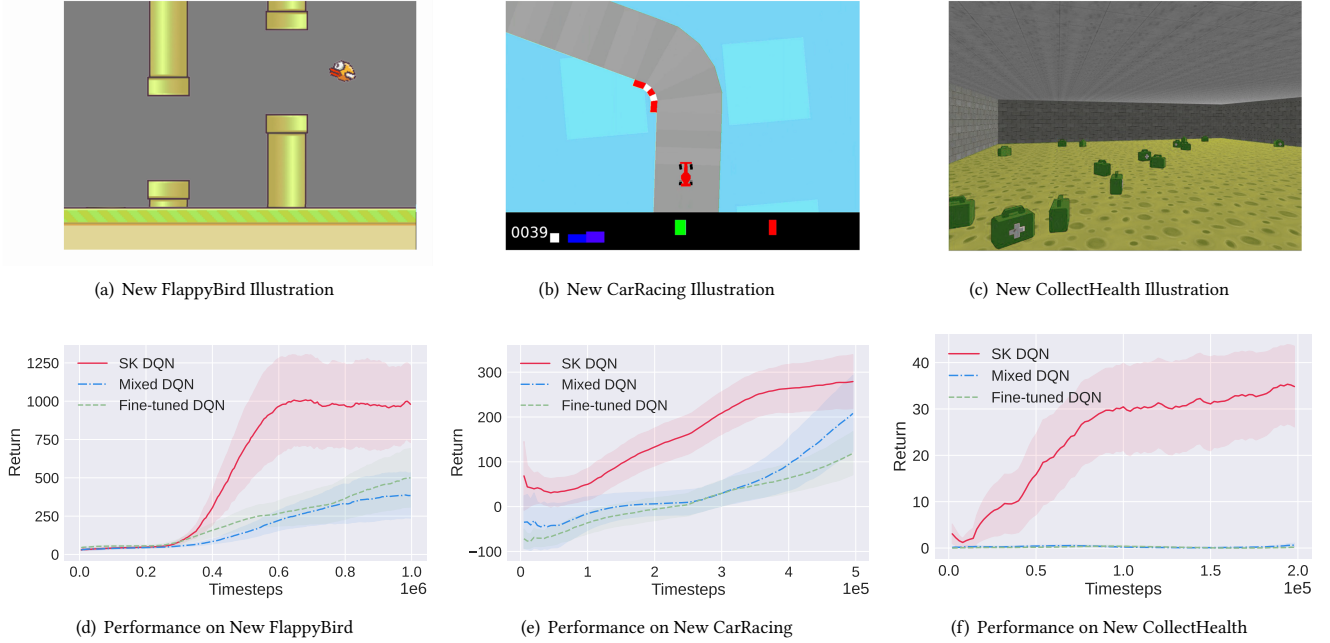
Figure 7: Three new RL environments and performance comparison of different methods.
