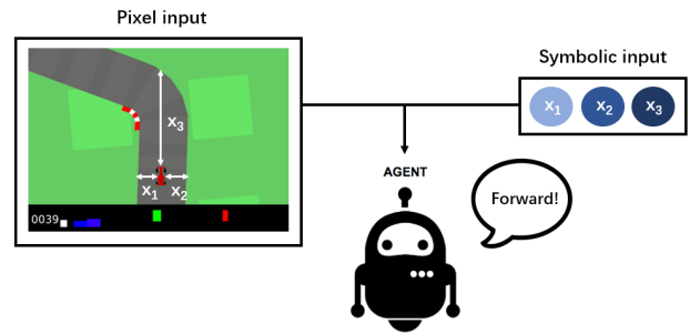
Figure 1: An illustration of the two forms of input in the self-driving car game.
