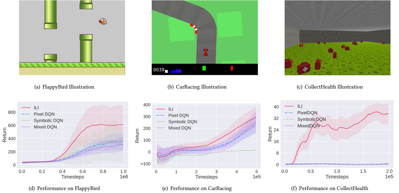
Figure 6: Three RL environments and performance comparison of different methods.
